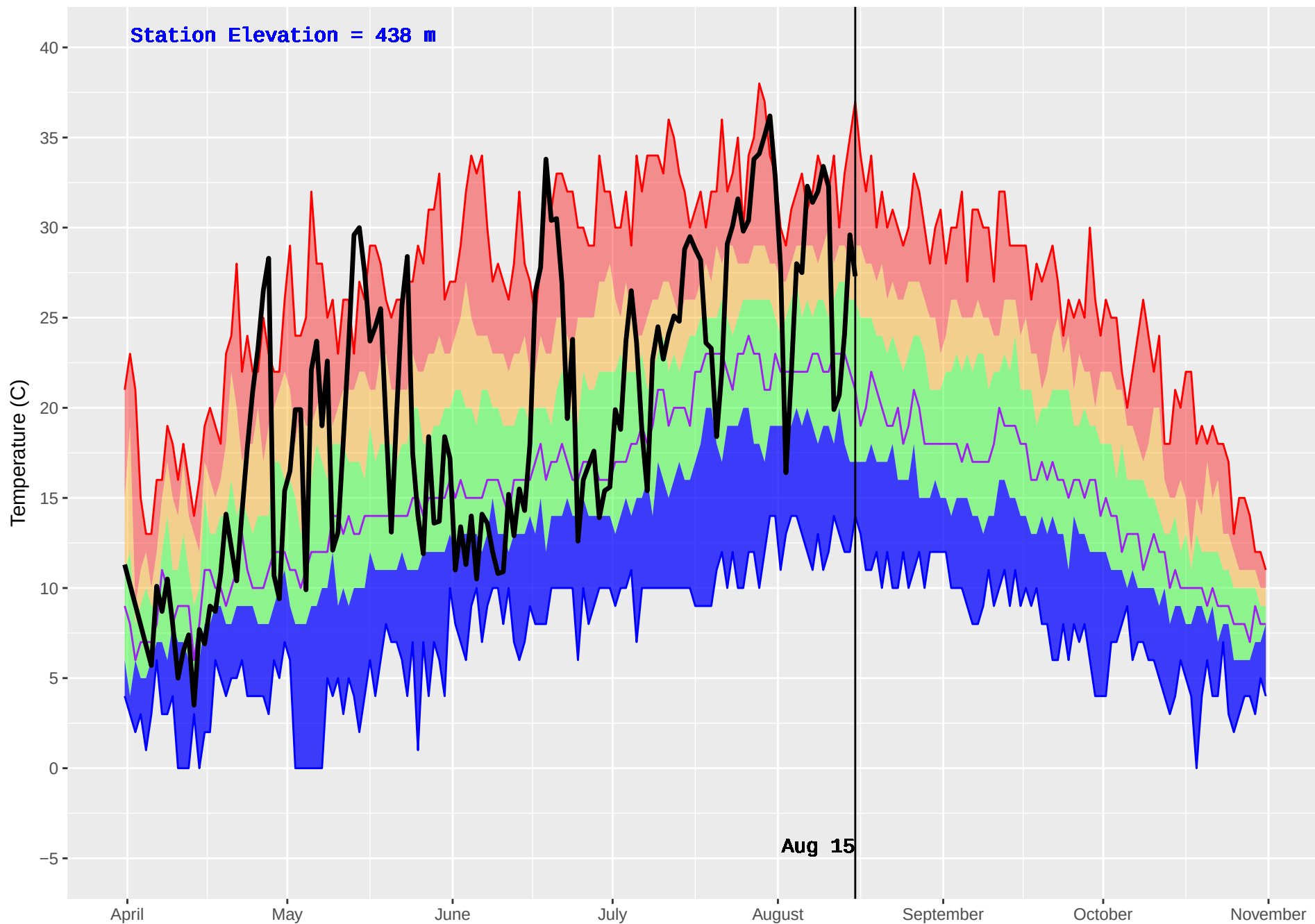
MENZIES CAMP (19) : Historical (1970–2016) and Current (2018) Daily Temperature
