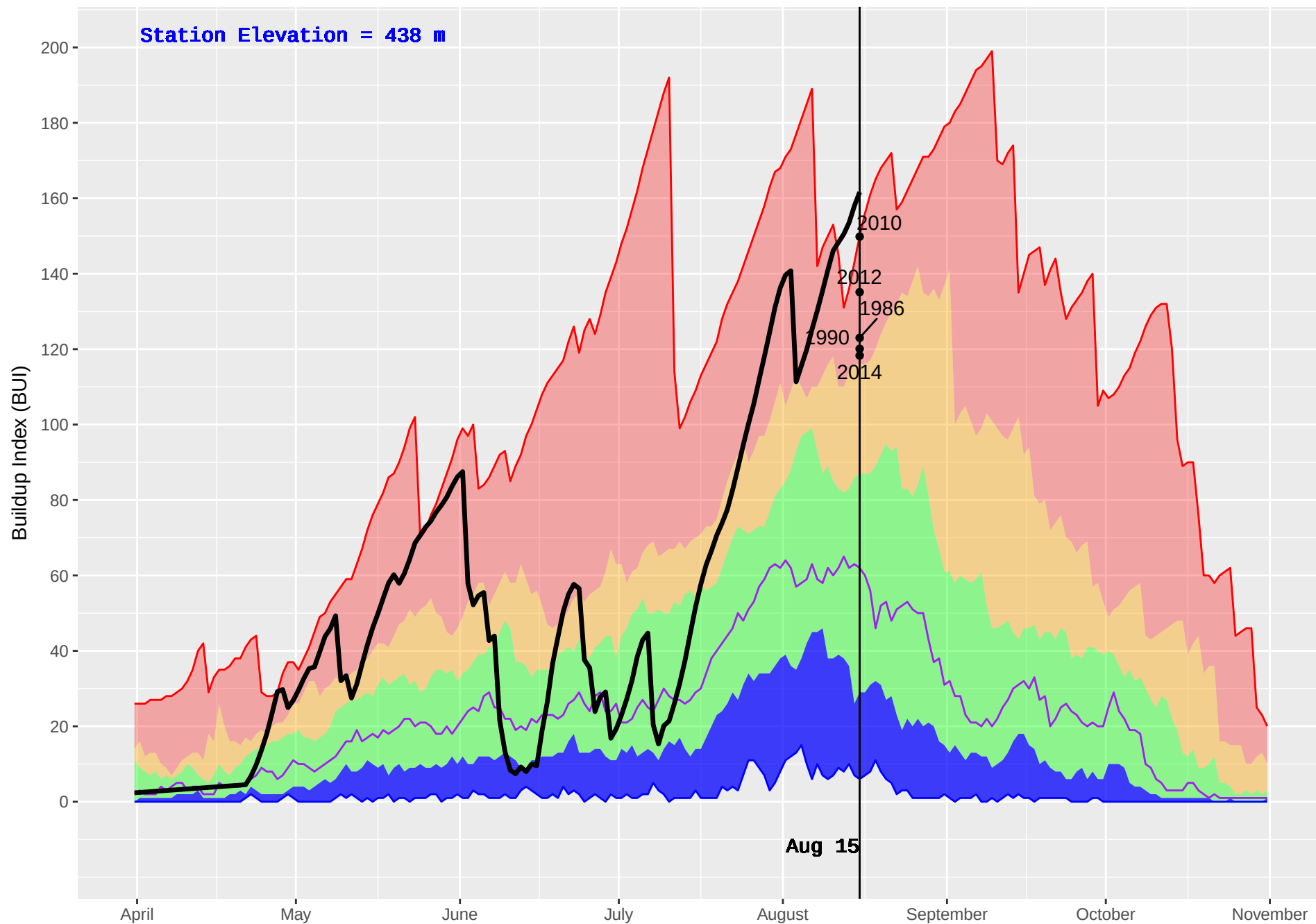
MENZIES CAMP (19) : Historical (1970–2016) and Current (2018) Daily Buildup Index (BUI)
