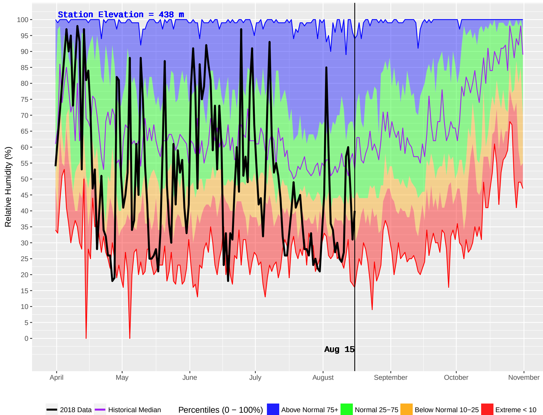
MENZIES CAMP (19) : Historical (1970–2016) and Current (2018) Daily Relative Humidity
