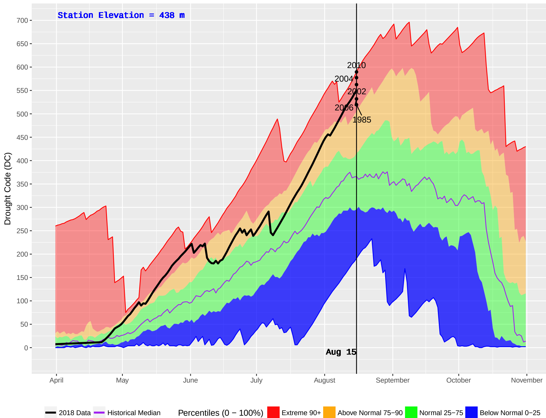
MENZIES CAMP (19) : Historical (1970–2016) and Current (2018) Daily Drought Code (DC)
